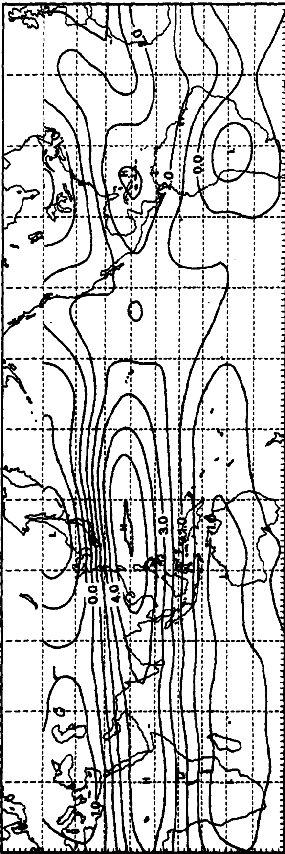
STREAM FUNCTION 200MB DEC AVG
